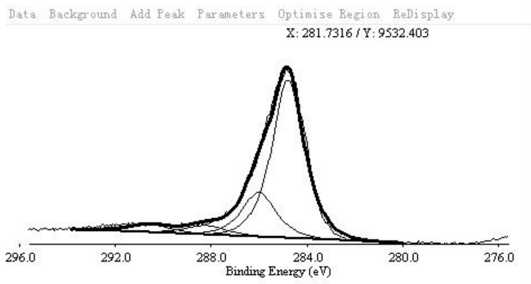
XPS
