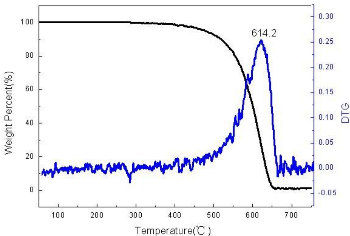
TG curve of short 8-15-COOH D101018
